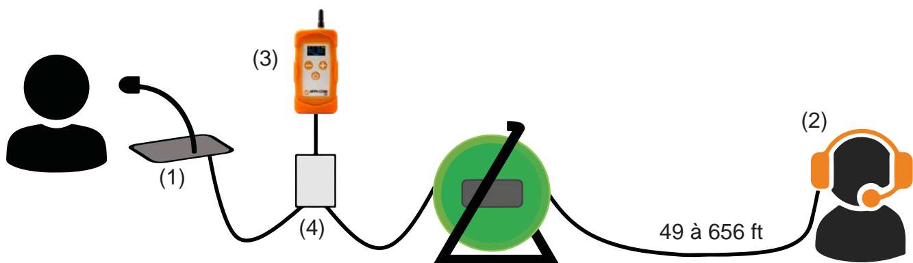
Desk (1) Audio devices (2). Intercom (3) Adapter box (4).
